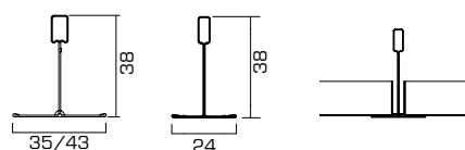
PLAN in appoggio lay - in tiles
